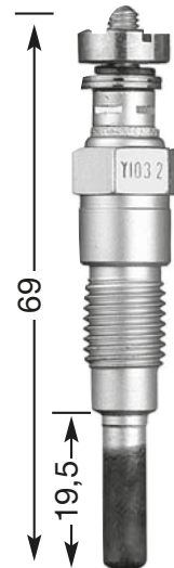
Y-103-2A M 10 x 1.25 12 Hex
