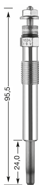
Y-524 J M 10 x 1.0 10 Hex 10 V DP 27
