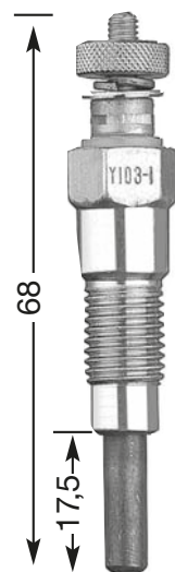
Y-103-1 M 10 x 1.25 12 Hex
