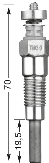
Y-103-2 M 10 x 1.25 12 Hex
