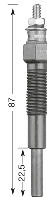
Y-157 R M 10 x 1.25 12 Hex 23 V
