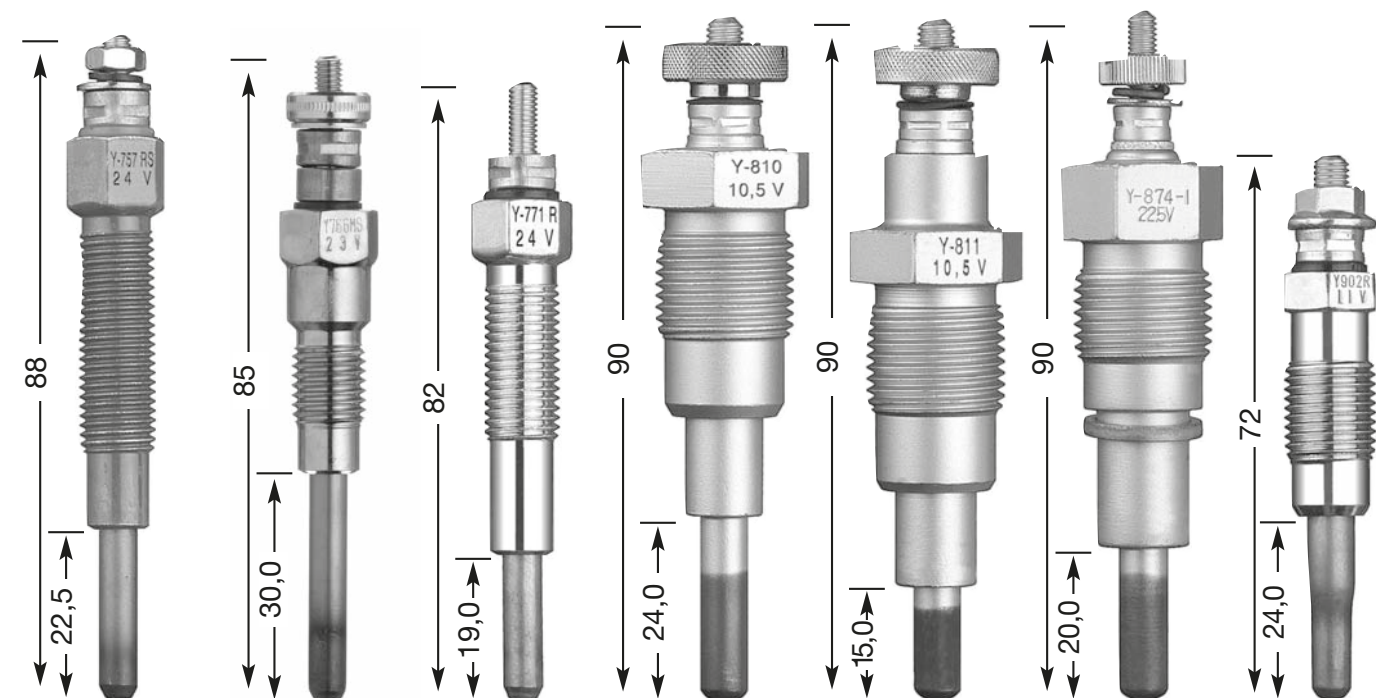
Y-757 RS M 10 x 1.25 12 Hex 24 V
